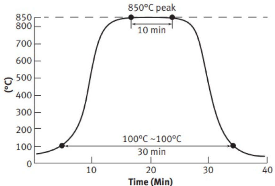
Micromax™ Standard QA Firing Profile ( 850^{\circ}\text{C} 10 min)
